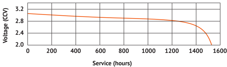
Service output test 7.5kΩ 24hrs/day
