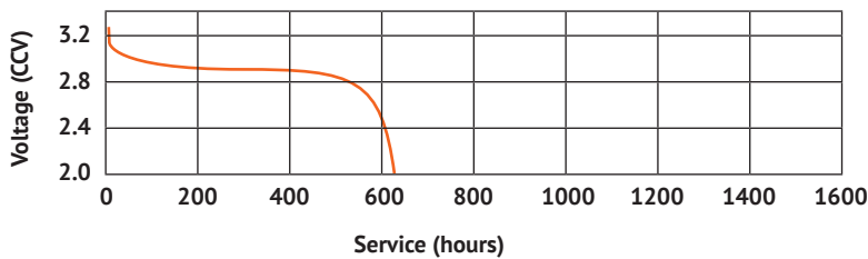
Service output test 15kΩ 24hrs/day
